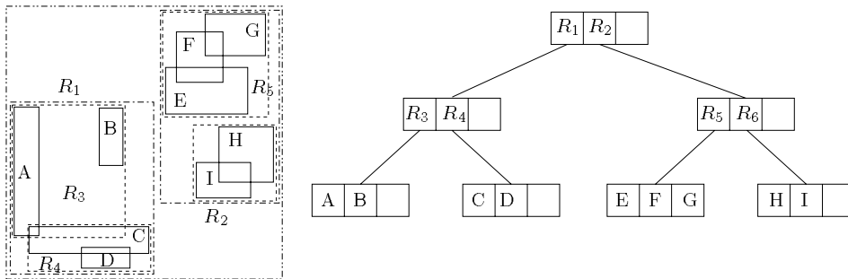
FIGURE 5. An R-tree.
