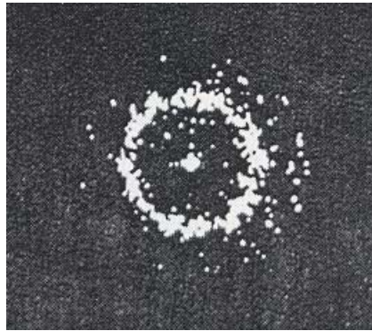
Fourier transform
